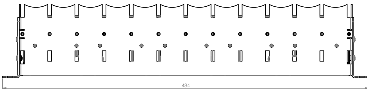
Dimensions (mm)
