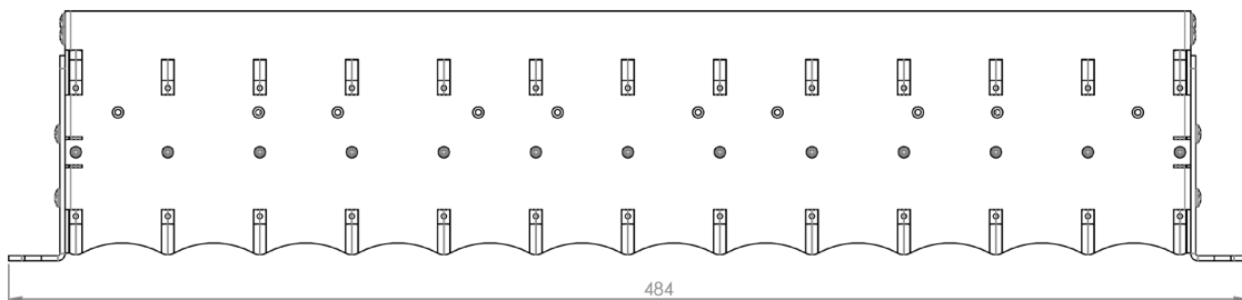
Dimensions (mm)
