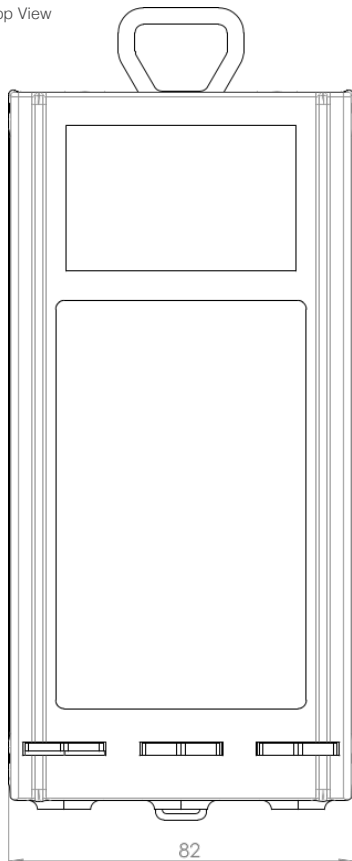
Dimensions (mm)
